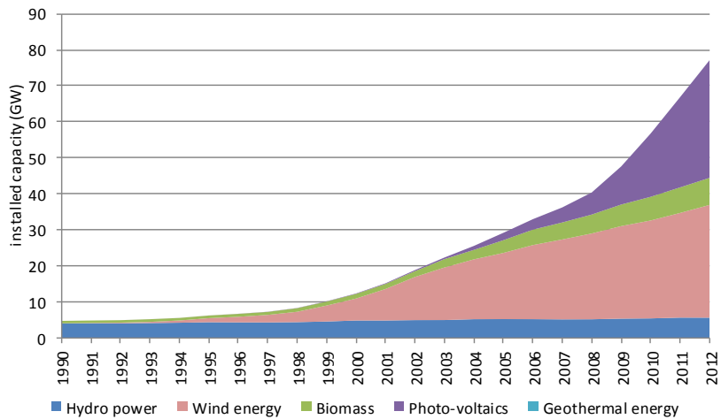
Figure 4: DG Installed capacity
