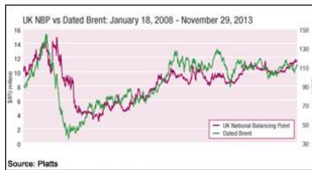
Figure 3 Relationship between oil and GB gas prices
