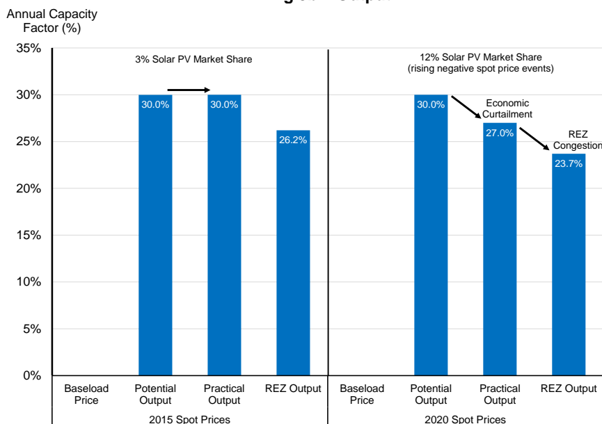
Fig.9b – Output
